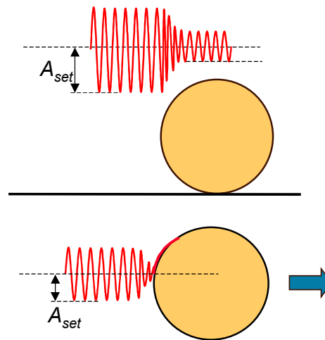
Fig.4 – Mechanically pushing a nanoparticle.
