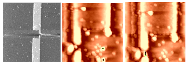
Fig. 8 – Building a single-electron transistor by nanomanipulation.
