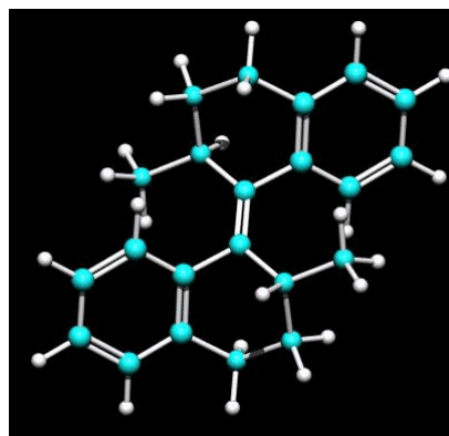
Fig. 1 – The central part of a rotary nanomachine. (Figure courtesy of Professor Ben L. Feringa's group.)
